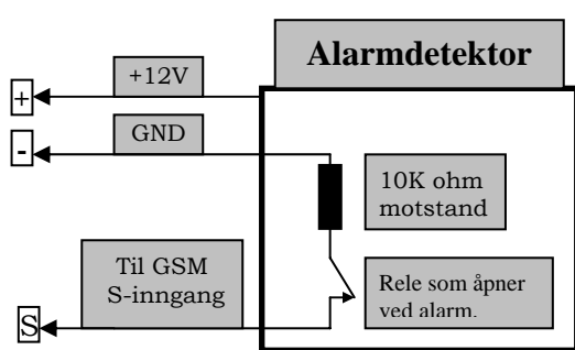
Figur 5: Alarmterminering Prinsippskisse
